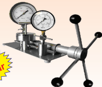
Pressure Calibrator - Water Operated Comparison Test Pump
